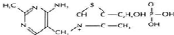
Thiamine monophosphate
